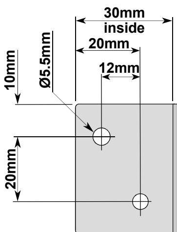
Swivel Mounting Bracket
