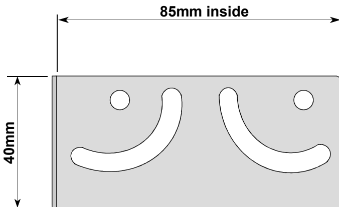
Swivel Mounting Bracket
